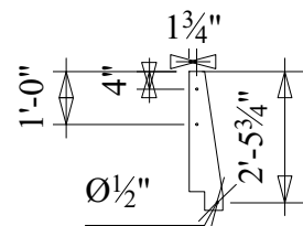
C4 Brace- Holes
