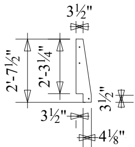
C2 Brace- Front
